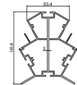
Aluminium Sectional View of Double Glass Model
