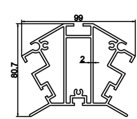
Aluminium Sectional View of Single Glass Model
