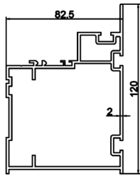
Aluminium Sectional View of Double Glass Model
