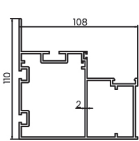
Aluminium Sectional View of Double Glass Model
